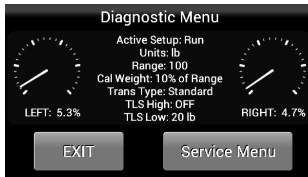
Figure 15 - DIAGNOSTIC DISPLAY
